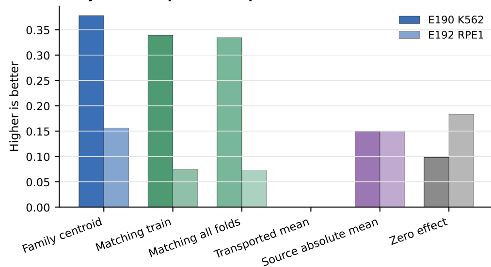
C Selected-gene centroid accuracy (effect space)
