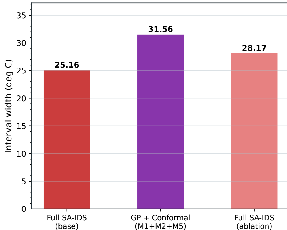
Prediction interval width
