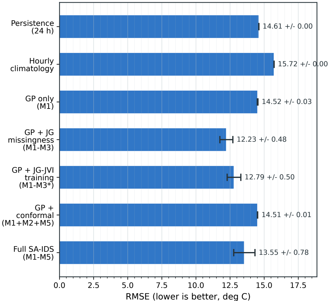
RMSE
