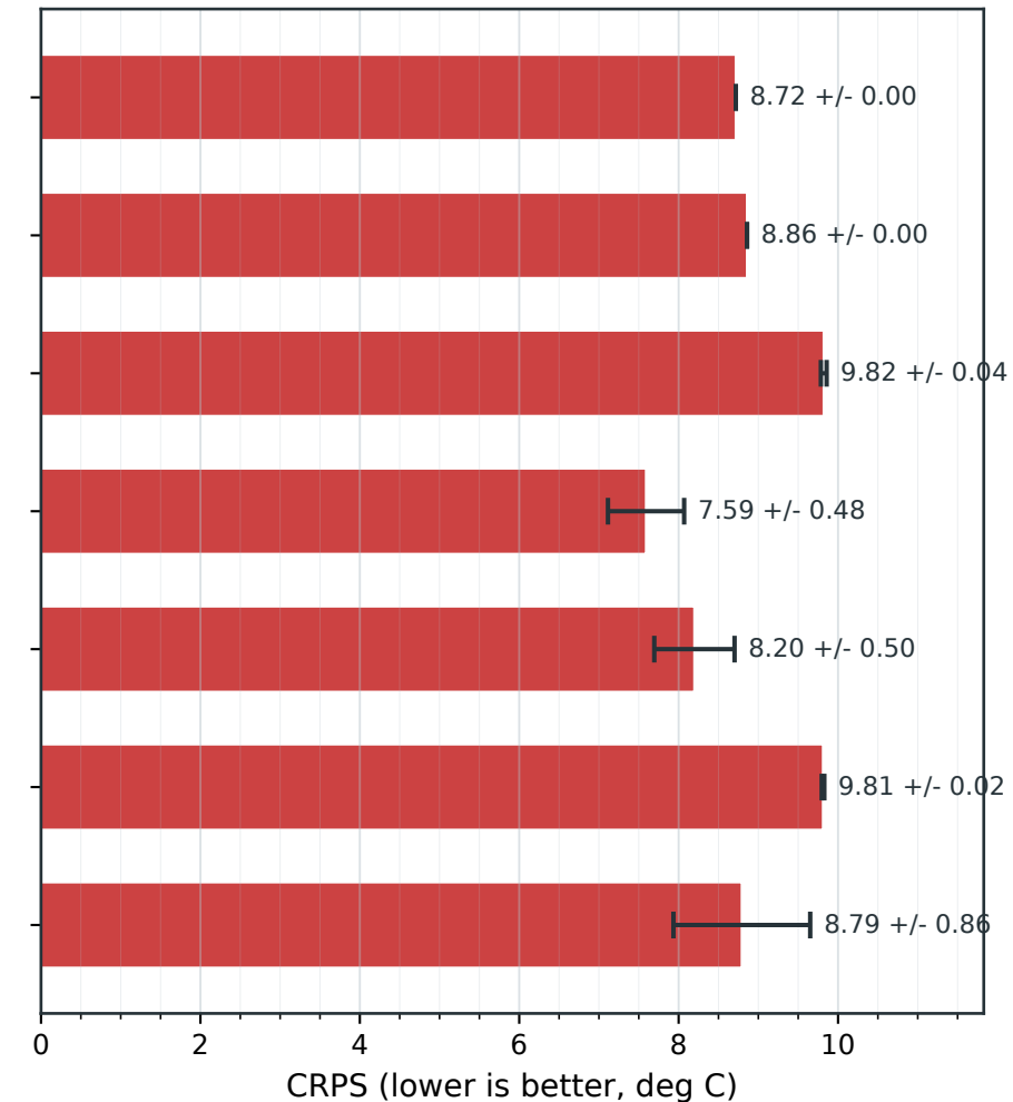
CRPS
