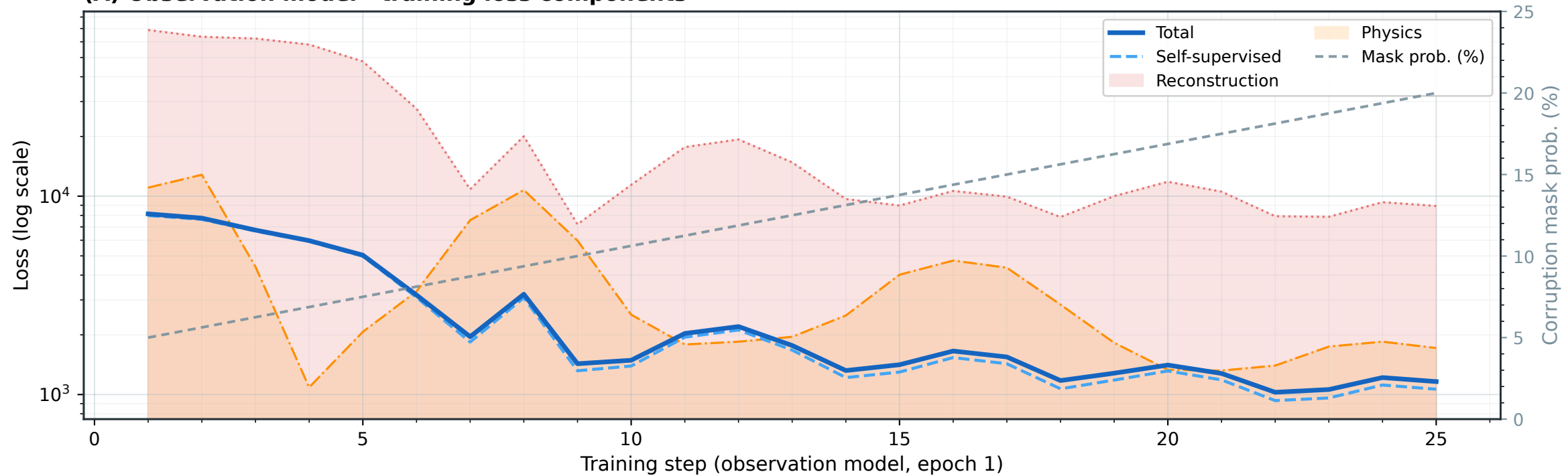
(A) Observation model - training loss components
