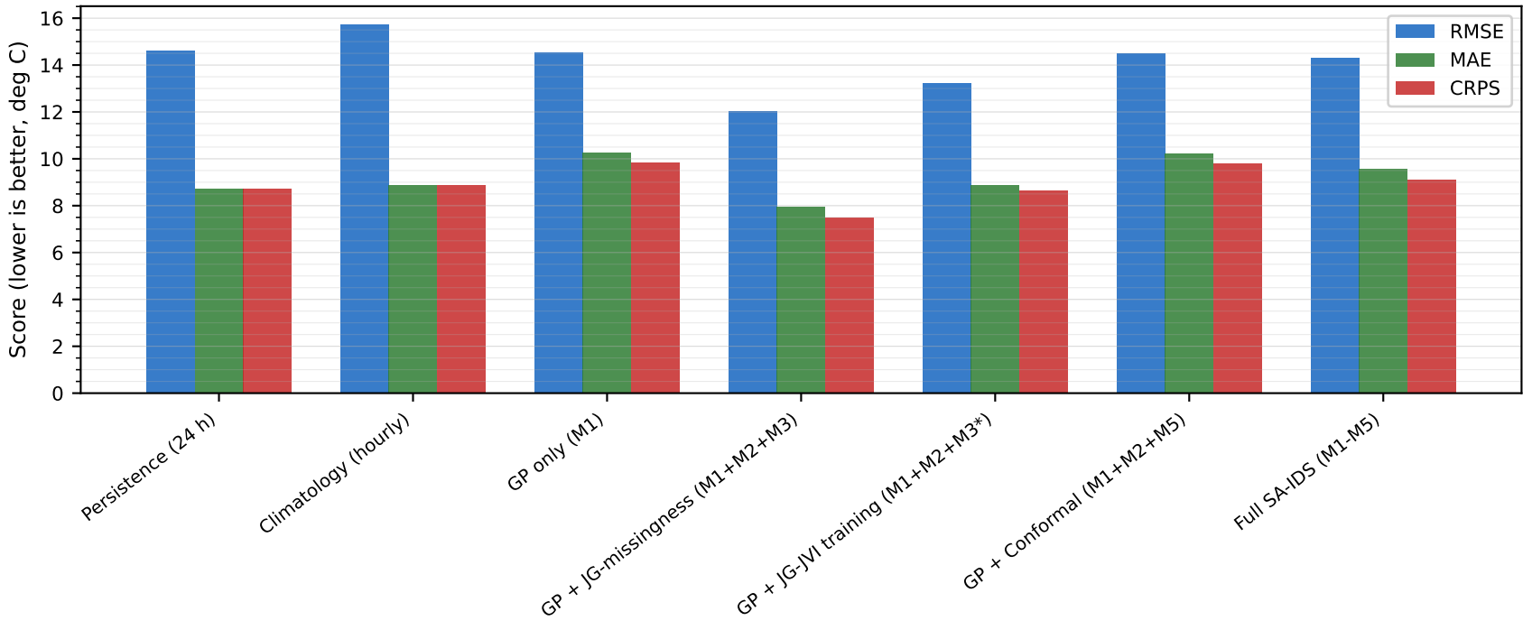
RMSE / MAE / CRPS by model variant — EMS patch v0.1.0
