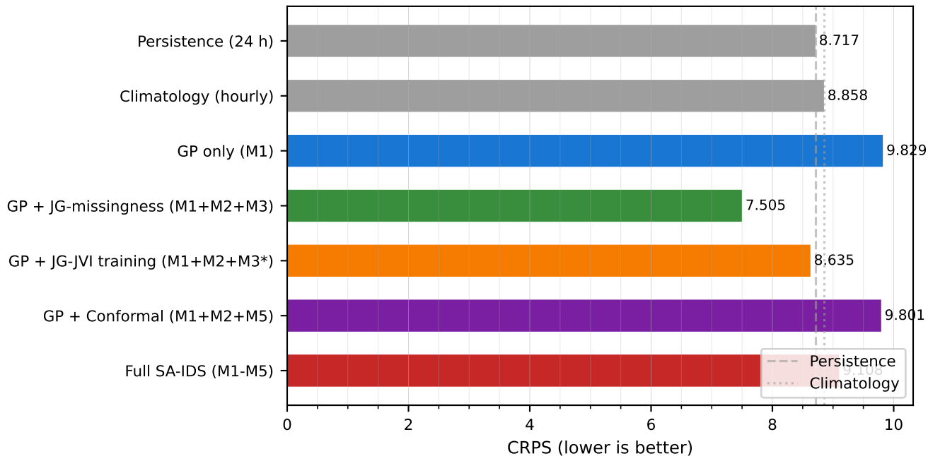
CRPS by model variant — EMS patch v0.1.0
