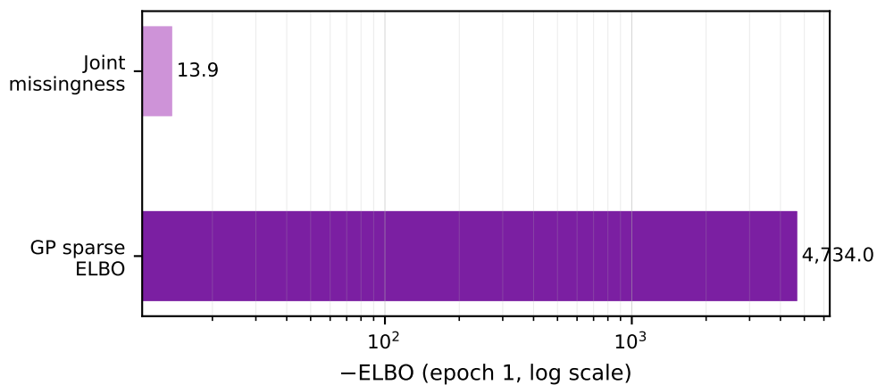
(B) State model [total: 4,747.9]
