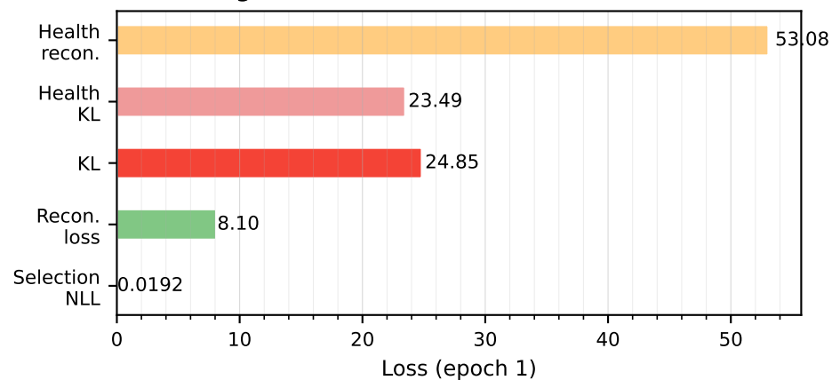
(C) Missingness ELBO [total: 13.91]
