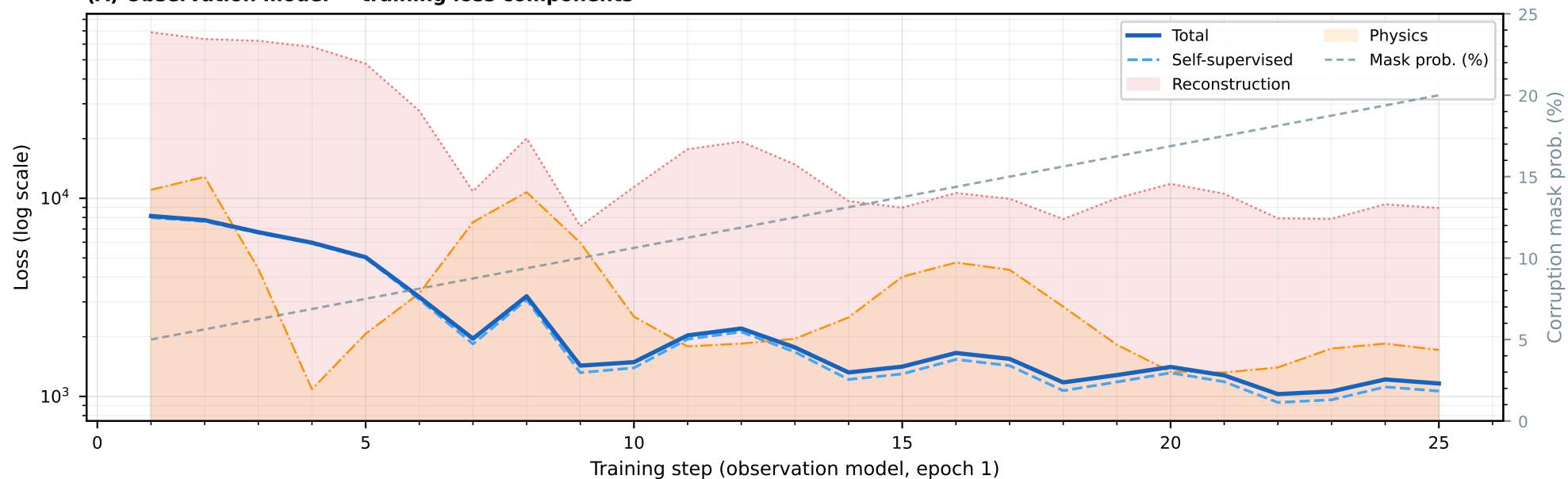
(A) Observation model — training loss components
