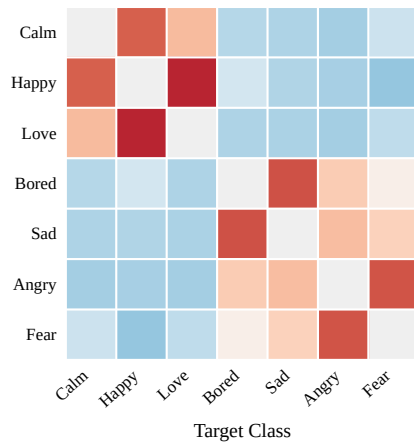
SPP-SCL
