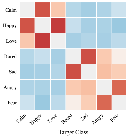
CLMLF
