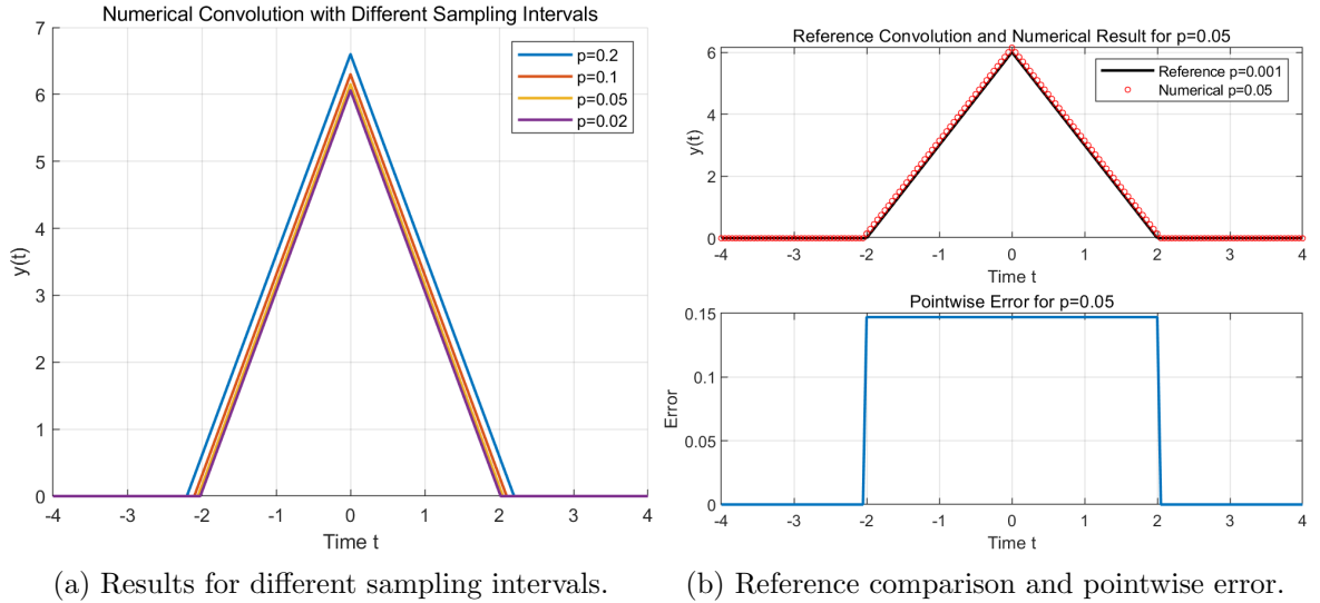
Figure 4: Numerical convolution results.
