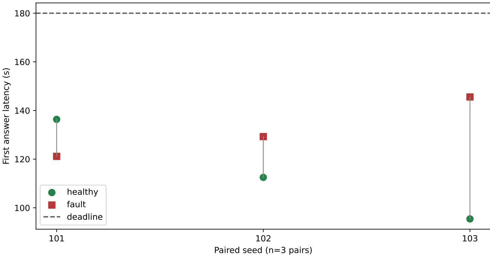
E4 first answer timing; every run ended FAIL5 / UNKNOWN1
