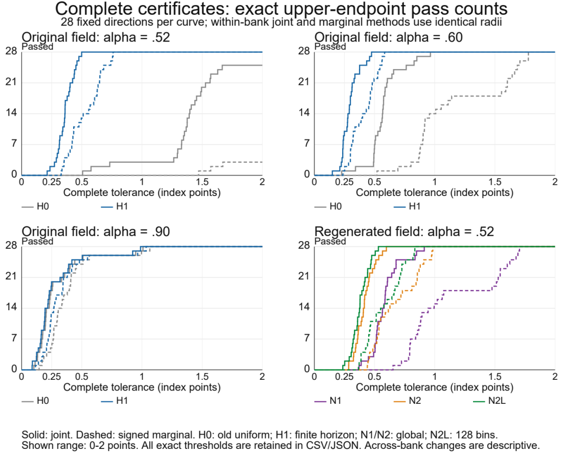
Figure E.1. Exact-threshold budget-pass-count curves; 28 fixed directions per configuration.
