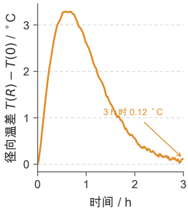
(c) 径向温差迅速衰减
