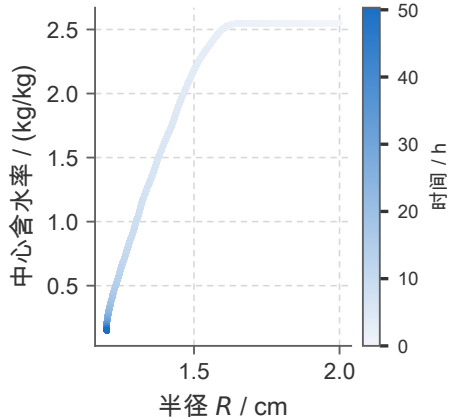
(c) 半径-含水率相轨
