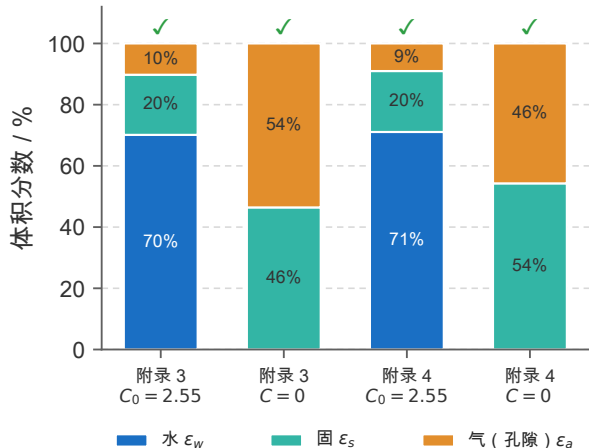
(b) 三相体积分数全程非负 ( \rho_s = 1400 )
