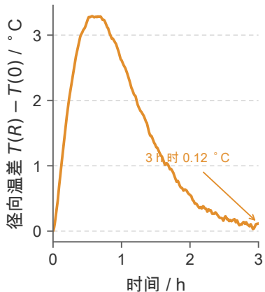
(c) 径向温差迅速衰减
