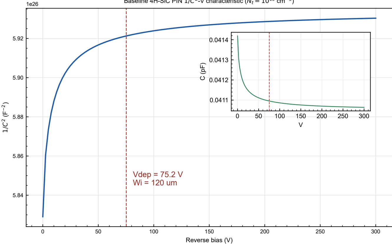
Baseline 4H-SiC PIN 1/C^2 -V characteristic ( N_t = 10^{13} \text{ cm}^{-3} )
