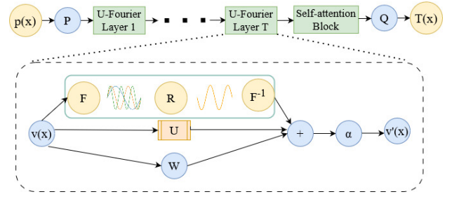
Fig. 1. Our SAU-FNO model architecture. p(x) is the input, P and Q are fully connected neural networks, and T(x) is the output. \mathcal{F} denotes the Fourier transform, R is the parameterization in Fourier space, \mathcal{F}^{-1} is the inverse Fourier transform, W is a linear bias term, and \alpha is the activation function. U denotes a U-Net.
