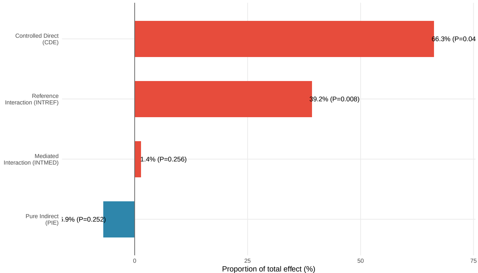
Figure 11. CMAverse 4-way decomposition: Se → GGT → LSM = 8 kPa
