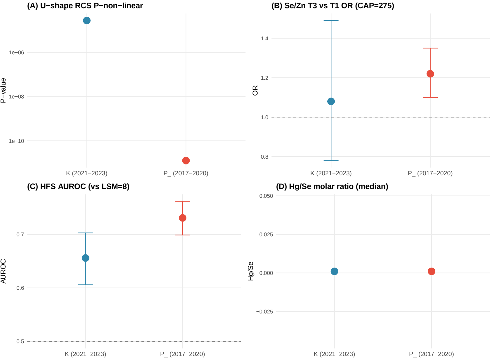
Figure 12. External validation: NHANES P_ (2017–2020) vs K cycle (2021–2023, design-weighted)
