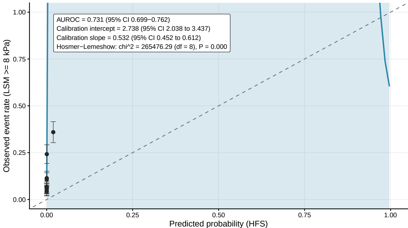
Figure 5. Hepamet HFS flexible calibration vs LSM \geq 8 kPa
