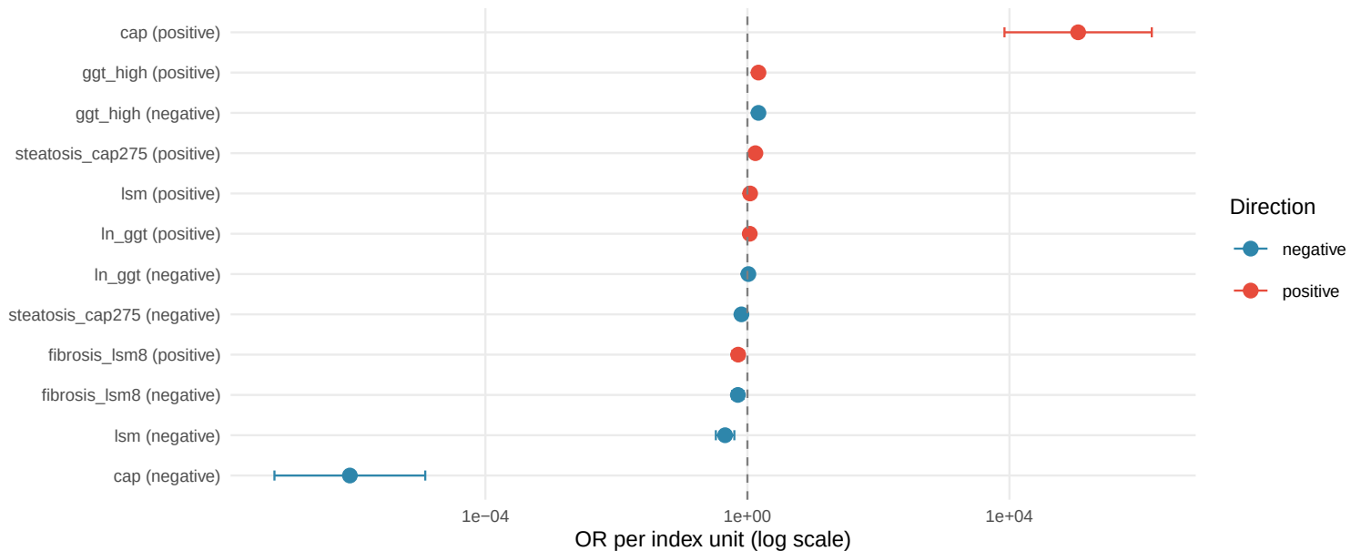
(B) WQS regression (OR per WQS-index increment)
