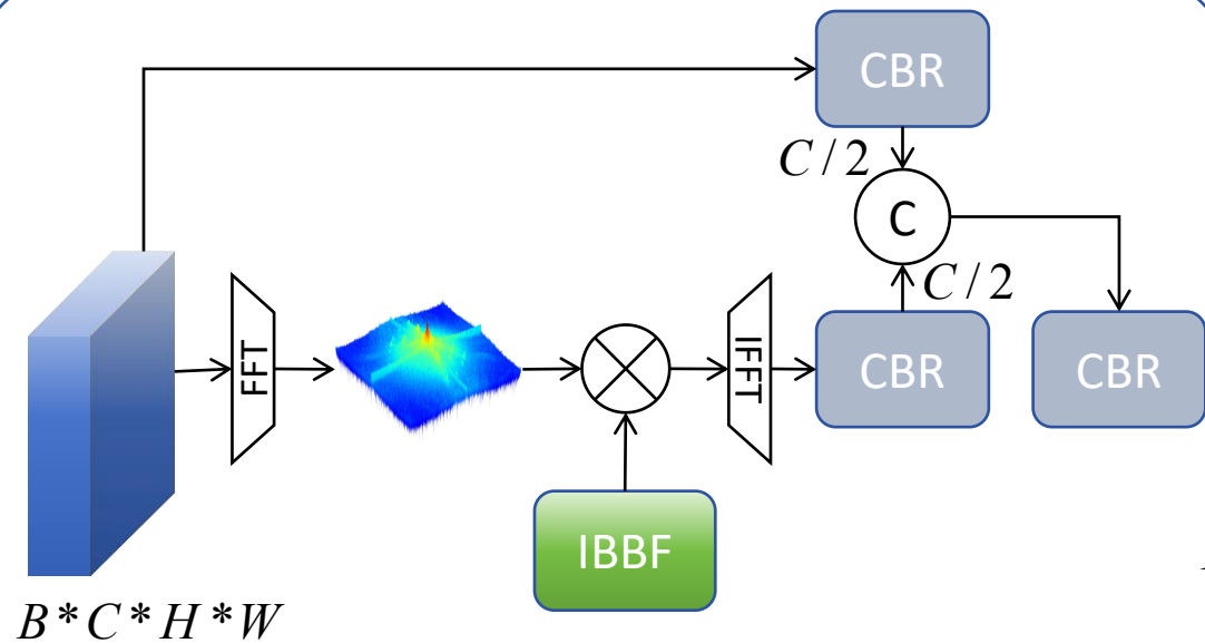
Improved Butterworth-Basis Filter
