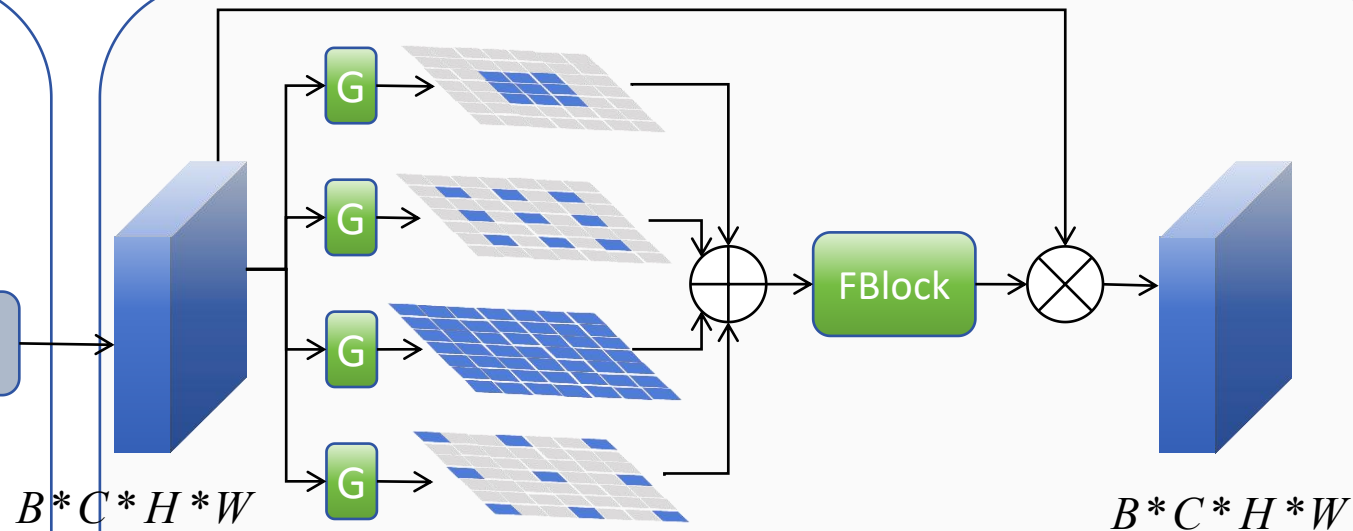
Multi-Receptive Field Depthwise Separable Channel Gating
