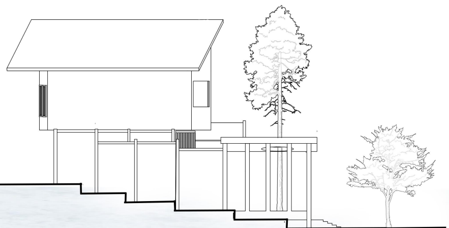
WEST ELEVATION VIEW 1:100
