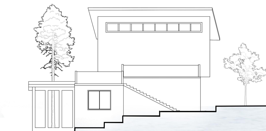
EAST ELEVATION VIEW 1:100
