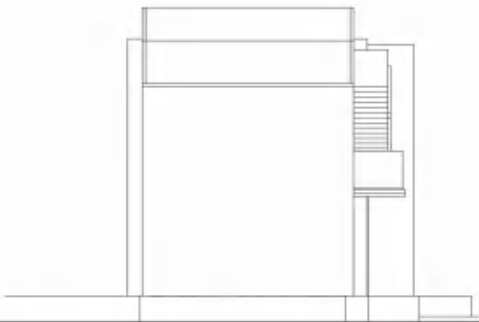
North Elevation 1:100
