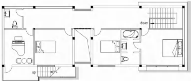
First Floor Plan 1:100
