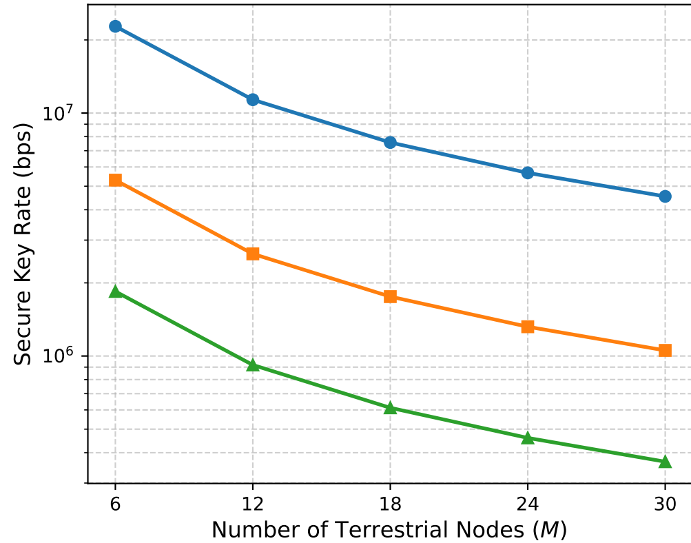
System Uniform SKR
