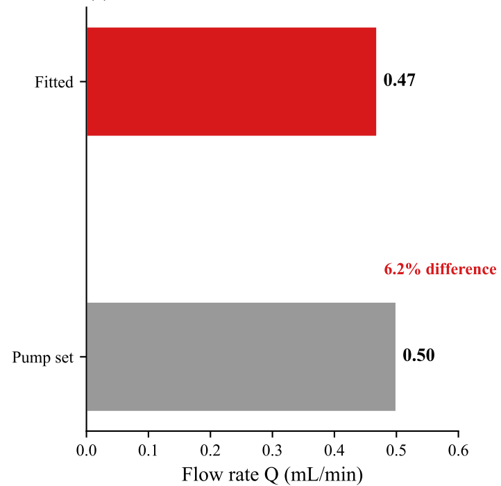
(c) Flow rate validation
