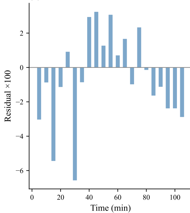
(b) Residuals
