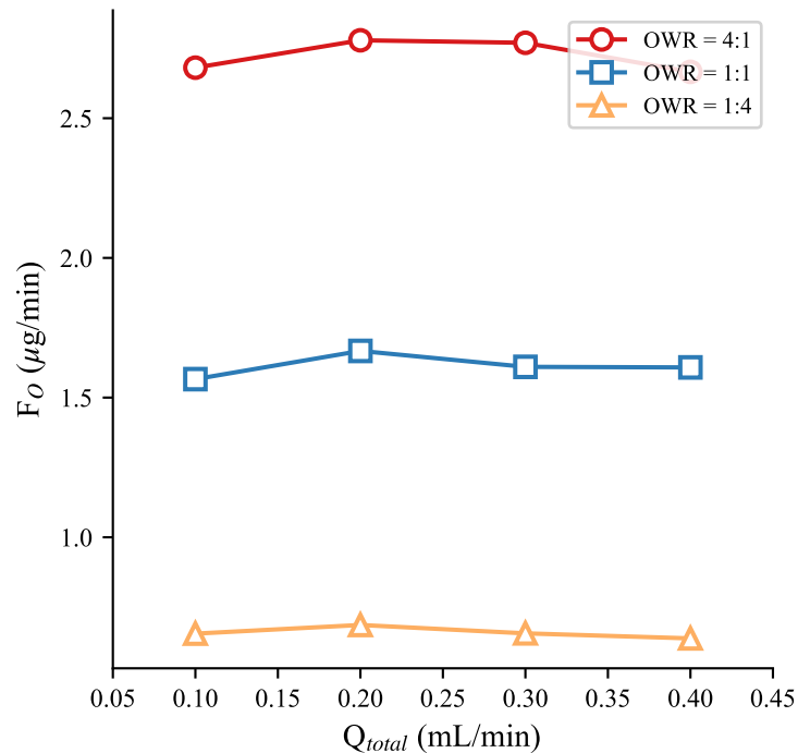
(b) Tracer flux vs. flow rate
