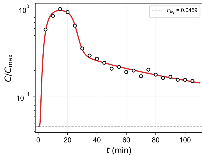
(b) Tail decay (log scale)
