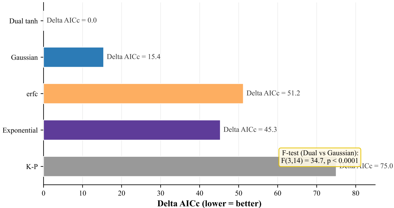
Figure 3: Model Comparison
