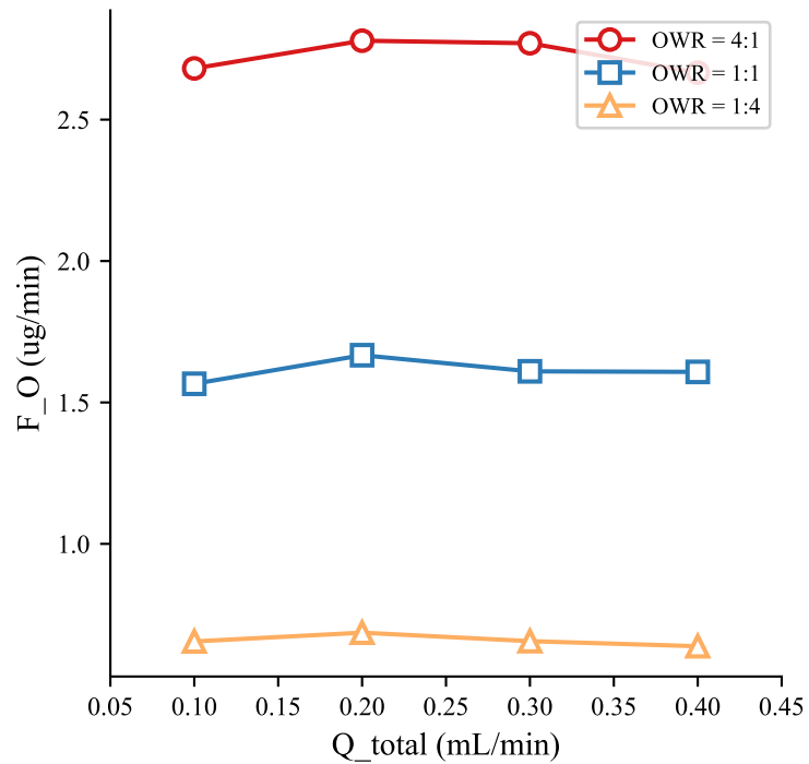
(b) Tracer flux vs. flow rate
