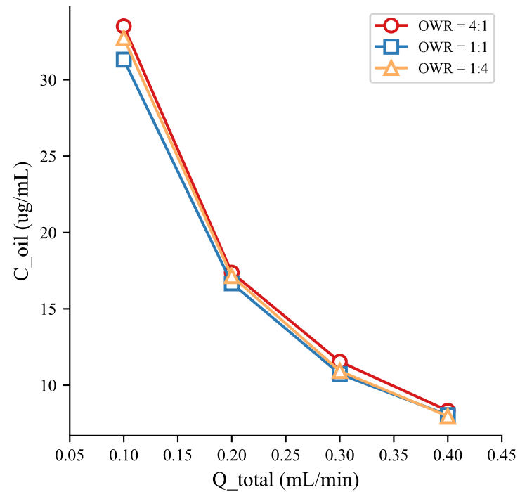
(a) Concentration vs. flow rate
