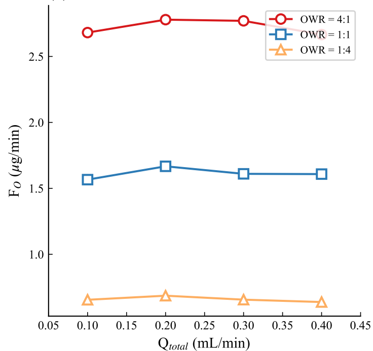
(b) Tracer flux vs. flow rate
