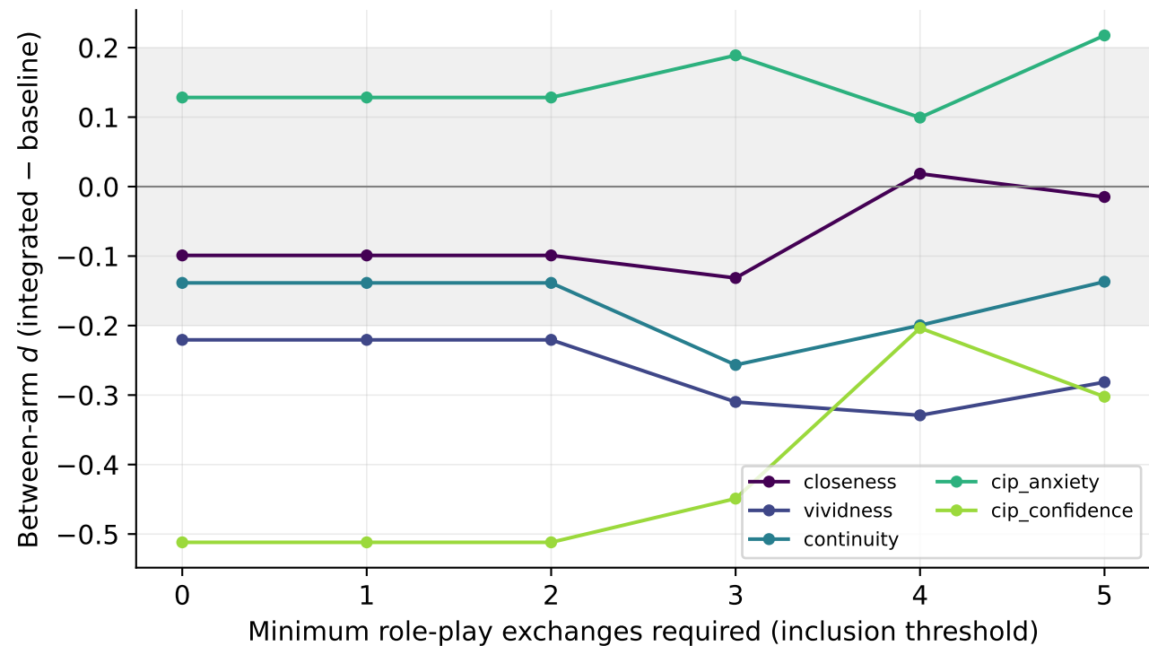
Figure E2. Sensitivity of between-arm effects to the minimum-turn threshold (0-5)
