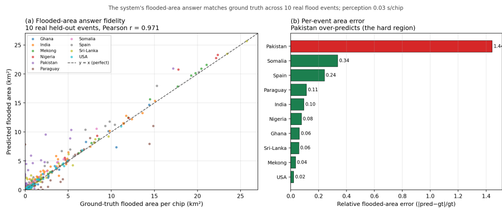
Fig. 7 End-to-end decision-level answer fidelity. Flooded-area answers produced by the full perception \rightarrow calibration \rightarrow reasoning agent against analyst hand-labels across 431 chips spanning ten real flood events (Pearson r = 0.971 ; Spearman \rho = 0.899 ; median absolute percentage error 25 %). The Pearson headline is driven by the largest events (bottom-50 %-by-area chip r = 0.118 ): the agent's totals are reliable in the event-ranking regime responders use, while small-area chips carry wide relative errors (deployment results).
