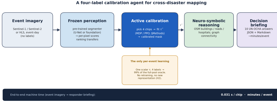
Fig. 2 System architecture of the calibration-centric agent. Event-day Sentinel-1/2 or HLS imagery is mapped by a frozen perception model (a trained U-Net or a frozen foundation backbone) whose per-pixel ranking transfers across events. The active-calibration stage — formalised as a Markov decision process and solved with PPO (Methods) — spends a four-chip label budget to recover the event-optimal decision threshold \tau^* , the only per-event learning in the pipeline; this single scalar recovers \approx 99\% of the full-pool oracle’s F1 with no retraining and no new representation (hypothesis H2). The calibrated binary mask is passed to a neuro-symbolic reasoning layer that queries OpenStreetMap buildings, roads and hospitals and runs graph-connectivity analysis to answer ten standard UN-OCHA emergency questions, emitted as a machine-auditable JSON briefing plus an analyst-readable summary. End-to-end machine time is dominated by perception (0.031 s per chip) and the OpenStreetMap query (minutes), not by any per-event training.
