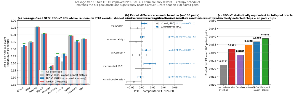
Fig. 3 Leakage-free leave-one-event-out evaluation of active threshold calibration. a , Per-event test F1 of the learned PPO policy before (v1, grey) and after (v2, blue) the three structural corrections (GAE- \lambda credit assignment, episode-terminal reward, entropy schedule), against four-chip random calibration (red) and the full-pool oracle (green dashes); shaded bands show the base-to-oracle calibration headroom per event. b , Pooled paired differences (PPO minus comparator) with 95% confidence intervals across the leave-one-event-out protocol. c , Pooled F1 ladder across all methods. The five practical 4-chip selection methods span only 0.017 F1 — an order of magnitude smaller than the single-event calibration drift (up to +0.235 F1) that any of them corrects.
