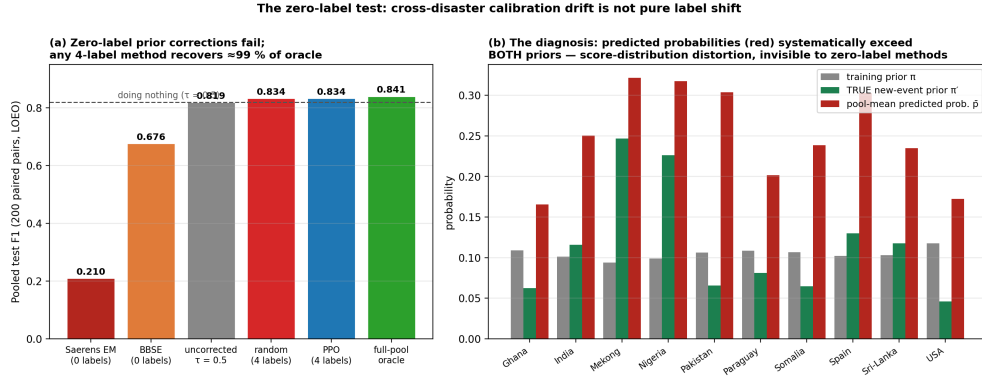
Fig. 5 The zero-label test: cross-disaster calibration drift is not pure label shift. a , Pooled test F1 (200 leave-one-event-out paired pairs) for the two standard zero-label prior-shift corrections — Saerens expectation-maximisation (EM) and black-box shift estimation (BBSE) — against the uncorrected default, four-label calibration, and the full-pool oracle. Both zero-label corrections fall below doing nothing. b , The diagnosis: per event, the model’s pool-mean predicted probability (red) systematically exceeds both the training prior (grey) and the true new-event prior (green). The class-conditional score distributions distort under cross-event transfer; labels measure this distortion, which no zero-label method can see. BBSE estimates the new-event priors nearly correctly yet its analytically corrected threshold still fails, isolating score distortion — not prior mis-estimation — as the dominant failure mode.
