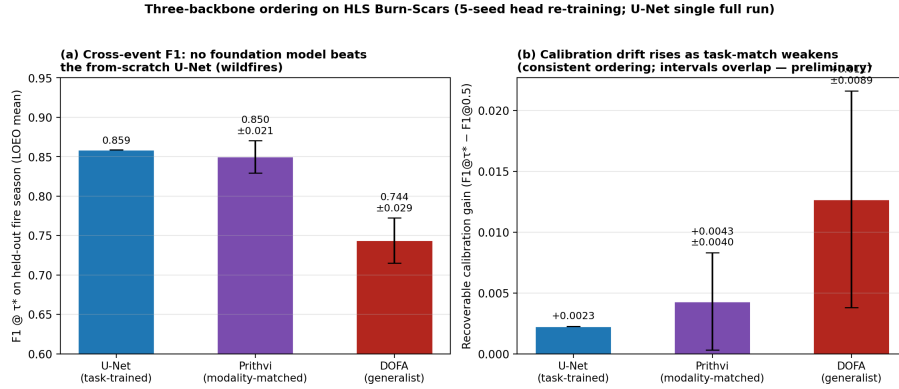
Fig. 6 Three-backbone ordering on HLS Burn-Scars: weaker task-match, more calibration drift. a , Cross-event F1 at the event-optimal threshold for a task-trained U-Net, the modality-matched Prithvi-EO-1.0-100M foundation model, and the generalist DOFA foundation model, under identical leave-one-fire-season-out protocols (foundation-model bars: mean \pm s.d. over five segmentation-head training seeds on frozen encoder features; U-Net: single full training run per fold). b , Recoverable calibration gain per backbone. The ordering is consistent across seeds but adjacent intervals overlap; we present it as a consistent preliminary ordering rather than a statistically separated gradient.
