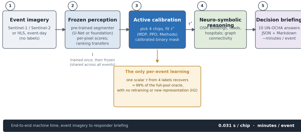
Fig. 2 System architecture of the calibration-centric agent. Event-day Sentinel-1/2 or HLS imagery is mapped by a frozen perception model (a trained U-Net or a frozen foundation backbone) whose per-pixel ranking transfers across events. The active-calibration stage — formalised as a Markov decision process and solved with PPO (Methods) — spends a four-chip label budget to recover the event-optimal decision threshold \tau^* , the only per-event learning in the pipeline; this single scalar recovers \approx 99\% of the full-pool oracle’s F1 with no retraining and no new representation (hypothesis H2). The calibrated binary mask is passed to a neuro-symbolic reasoning layer that queries OpenStreetMap buildings, roads and hospitals and runs graph-connectivity analysis to answer ten standard UN-OCHA emergency questions, emitted as a machine-auditable JSON briefing plus an analyst-readable summary. End-to-end machine time is dominated by perception (0.031 s per chip) and the OpenStreetMap query (minutes), not by any per-event training.
