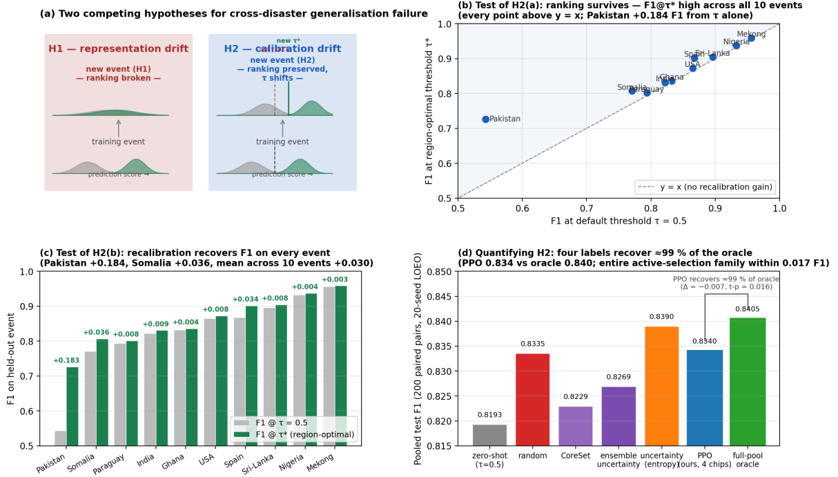
Figure 1: Two competing hypotheses for cross-disaster generalisation failure, and the experiments that discriminate them. a , Conceptual schematic. Under representation drift (H1, red) the per-class score distributions of a model applied to a new event collapse onto one another — the pixel ranking itself breaks, and no threshold can recover performance. Under calibration drift (H2, blue) the per-class distributions retain their shape but translate along the score axis — the ranking is preserved and a single threshold adjustment (from the training value \tau = 0.5 to the event-optimal \tau^* ) recovers performance. b , Test of H2(a): F1 at the event-optimal threshold versus F1 at the default threshold for the ten Sen1Floods11 flood events; every point lies above the identity line (Pakistan +0.184 F1 from the threshold alone). c , Test of H2(b): per-event F1 at \tau = 0.5 (grey) versus \tau^* (green), annotated with the recoverable calibration gain. d , Quantifying H2: pooled test F1 across 200 leave-one-event-out paired pairs for seven calibration strategies; a four-chip calibration set recovers \approx 99\% of the full-pool oracle’s F1 regardless of the selection method.
