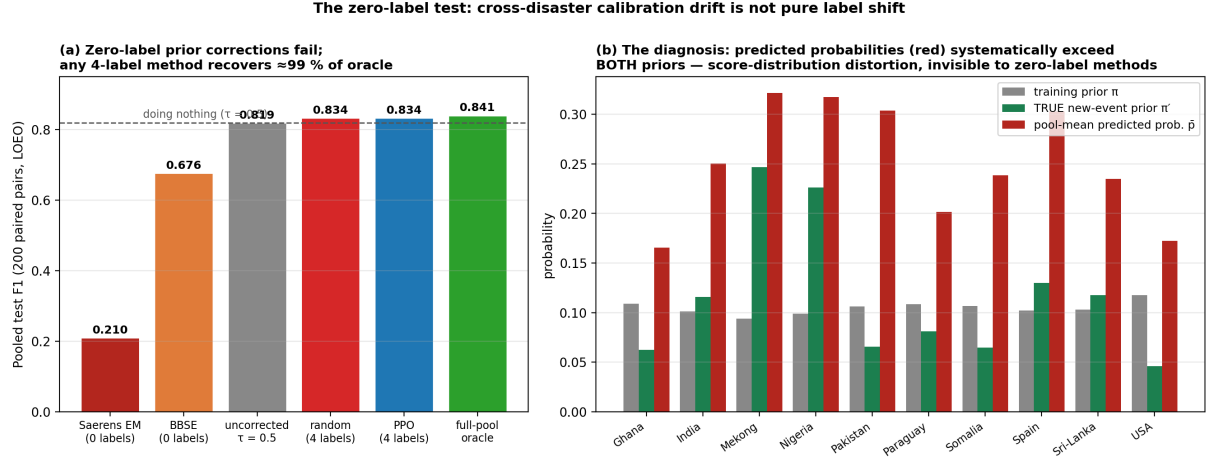
Figure 4: The zero-label test: cross-disaster calibration drift is not pure label shift. a , Pooled test F1 (200 leave-one-event-out paired pairs) for the two standard zero-label prior-shift corrections — Saerens expectation–maximisation (EM) and black-box shift estimation (BBSE) — against the uncorrected default, four-label calibration, and the full-pool oracle. Both zero-label corrections fall below doing nothing. b , The diagnosis: per event, the model’s pool-mean predicted probability (red) systematically exceeds both the training prior (grey) and the true new-event prior (green). The class-conditional score distributions distort under cross-event transfer; labels measure this distortion, which no zero-label method can see. BBSE estimates the new-event priors nearly correctly yet its analytically corrected threshold still fails, isolating score distortion — not prior mis-estimation — as the dominant failure mode.
