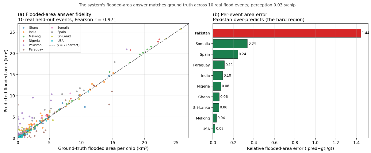
Figure 6: End-to-end decision-level answer fidelity. Flooded-area answers produced by the full perception \rightarrow calibration \rightarrow reasoning agent against analyst hand-labels across 431 chips spanning ten real flood events (Pearson r = 0.971 ; Spearman \rho = 0.899 ; median absolute percentage error 25 %). The Pearson headline is driven by the largest events (bottom-50 %-by-area chip r = 0.118 ): the agent's totals are reliable in the event-ranking regime responders use, while small-area chips carry wide relative errors (Results R1).
