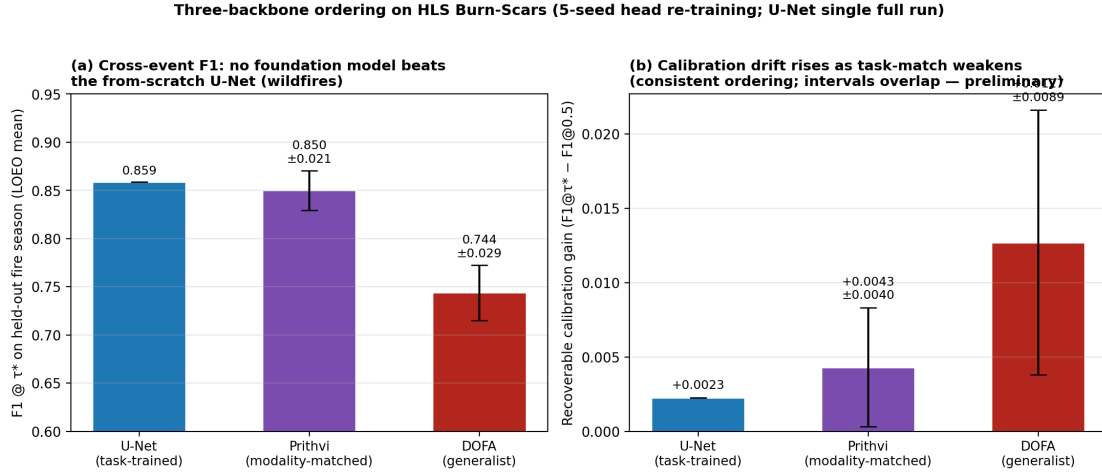
Figure 5: Three-backbone ordering on HLS Burn-Scars: weaker task-match, more calibration drift. a , Cross-event F1 at the event-optimal threshold for a task-trained U-Net, the modality-matched Prithvi-EO-1.0-100M foundation model, and the generalist DOFA foundation model, under identical leave-one-fire-season-out protocols (foundation-model bars: mean \pm s.d. over five segmentation-head training seeds on frozen encoder features; U-Net: single full training run per fold). b , Recoverable calibration gain per backbone. The ordering is consistent across seeds but adjacent intervals overlap; we present it as a consistent preliminary ordering rather than a statistically separated gradient.
