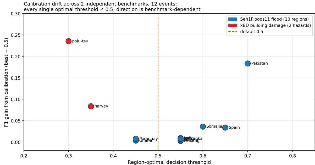
Figure 3: Calibration drift across benchmarks and hazard families. Event-optimal decision thresholds \tau^* and the F1 recovered by threshold re-fitting alone, for Sen1Floods11 floods and xBD building damage (HLS Burn-Scars wildfires reported in Results R3). The direction of drift is benchmark-specific (floods drift up, damage drifts down) and the magnitude is hazard-specific (large for floods and damage, small for wildfires), but 15 of 18 event-optimal thresholds differ from the 0.5 default.
