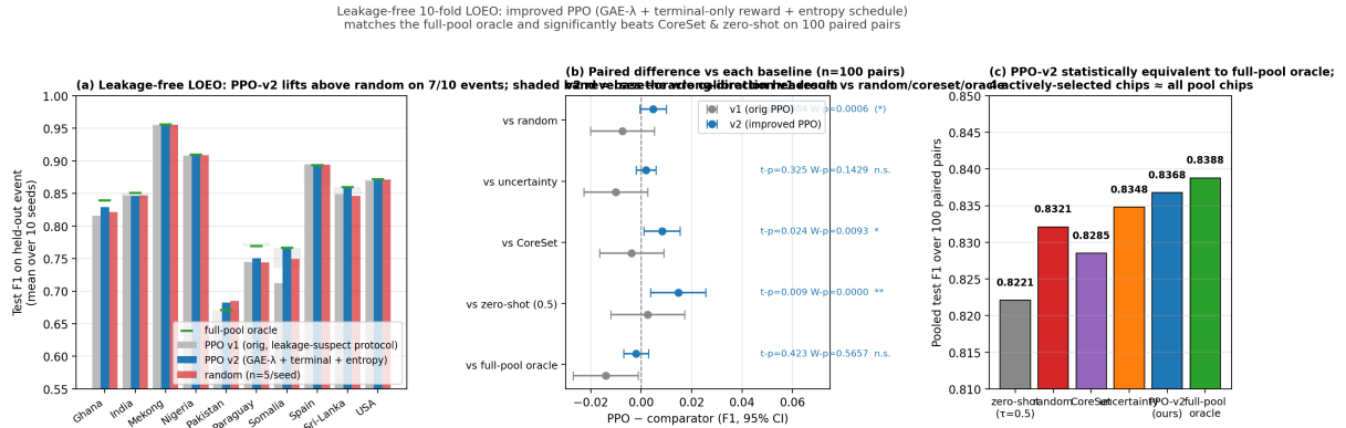
Figure 2: Leakage-free leave-one-event-out evaluation of active threshold calibration. a , Per-event test F1 of the learned PPO policy before (v1, grey) and after (v2, blue) the three structural corrections (GAE- \lambda credit assignment, episode-terminal reward, entropy schedule), against four-chip random calibration (red) and the full-pool oracle (green dashes); shaded bands show the base-to-oracle calibration headroom per event. b , Pooled paired differences (PPO minus comparator) with 95 % confidence intervals across the leave-one-event-out protocol. c , Pooled F1 ladder across all methods. The five practical 4-chip selection methods span only 0.017 F1 — an order of magnitude smaller than the single-event calibration drift (up to +0.235 F1) that any of them corrects.
