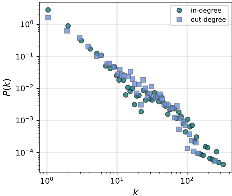
PolBlogs Degree Distribution
