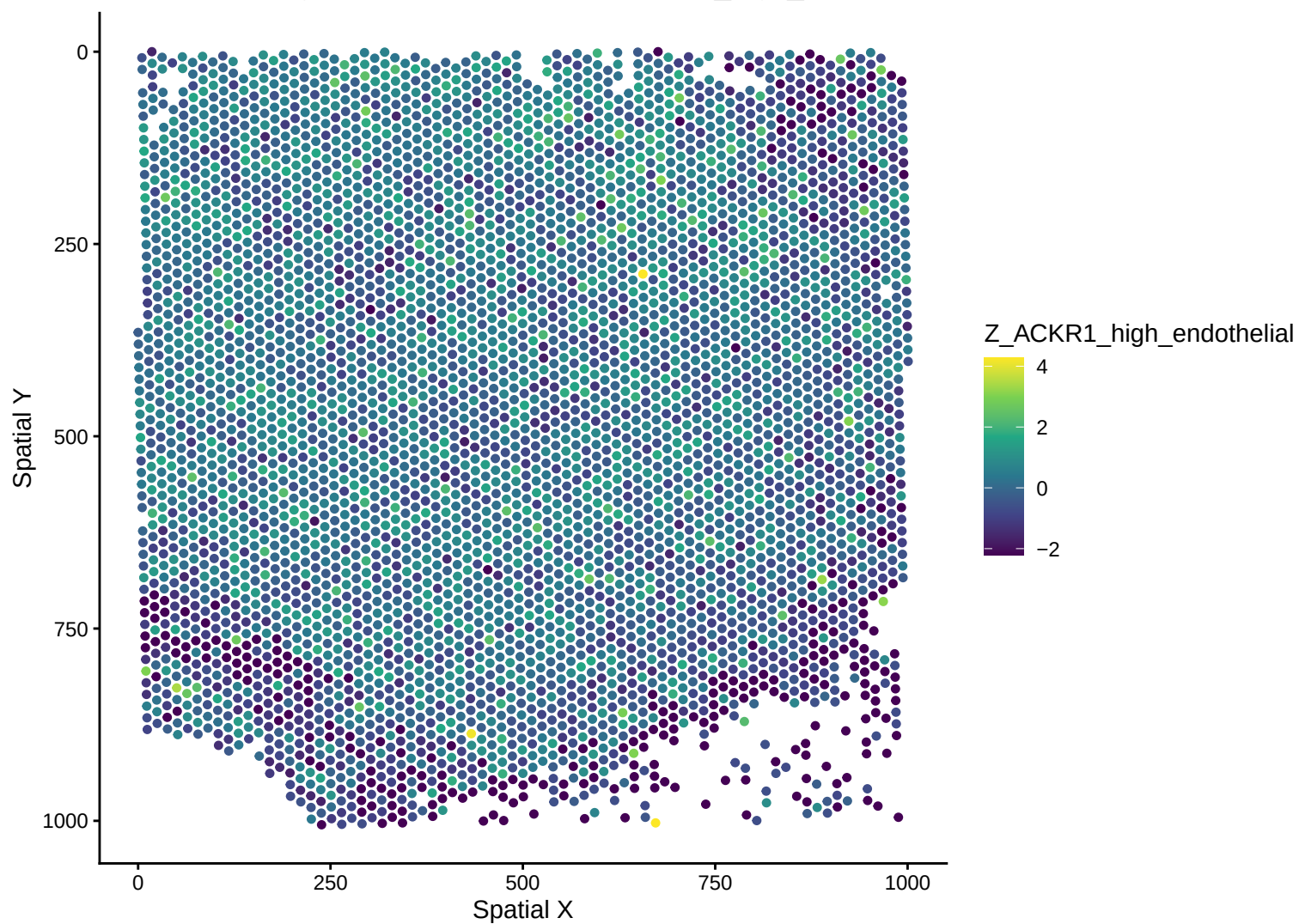
GSE206528 Signature in GSE261085: ACKR1_high_endothelial
