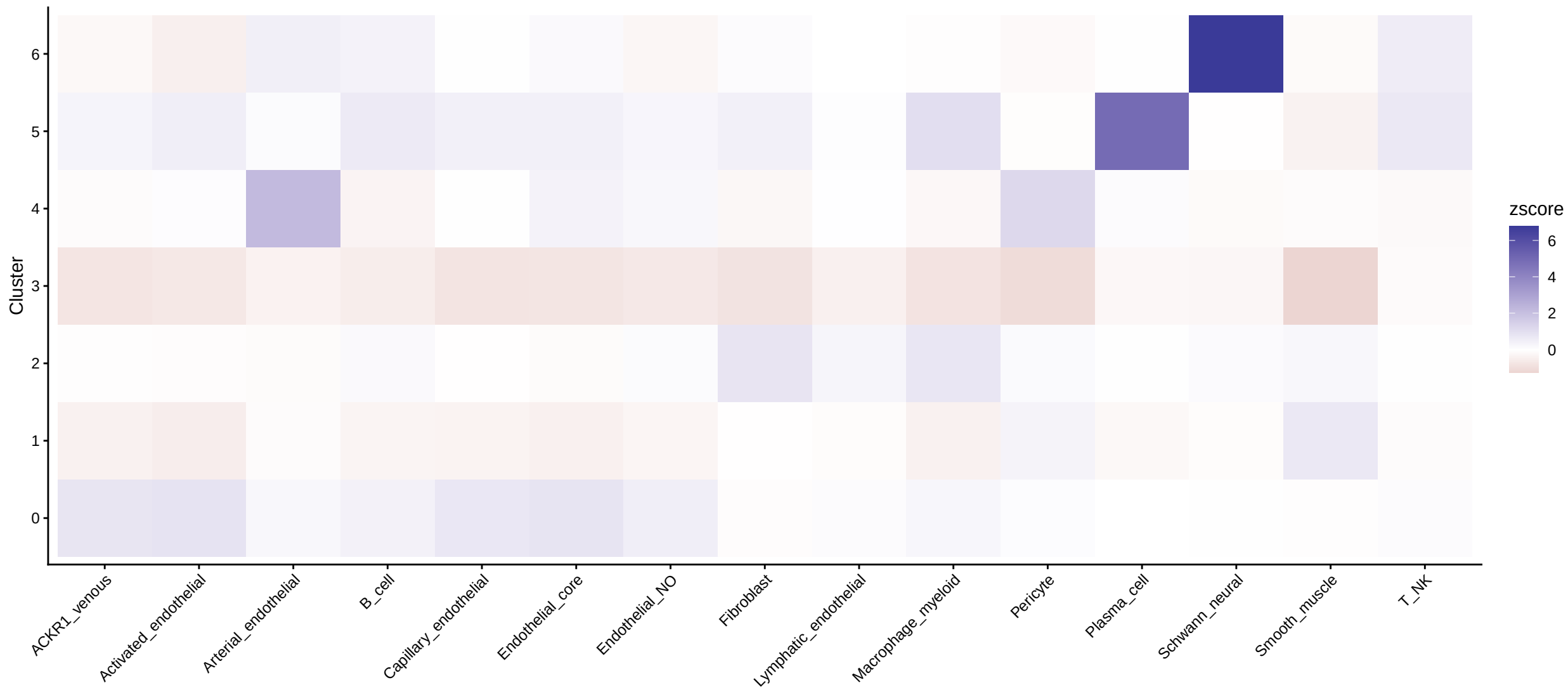
GSE261085 L13 Cluster Signature Enrichment
