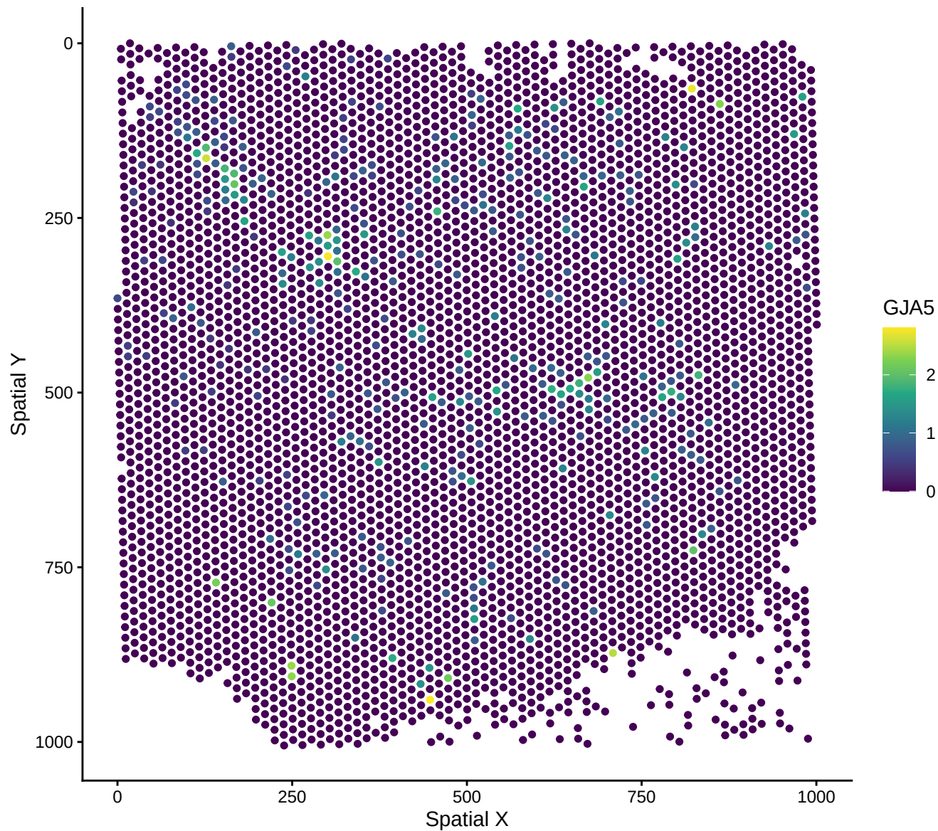
GSE261085 L13 Spatial Expression: GJA5
