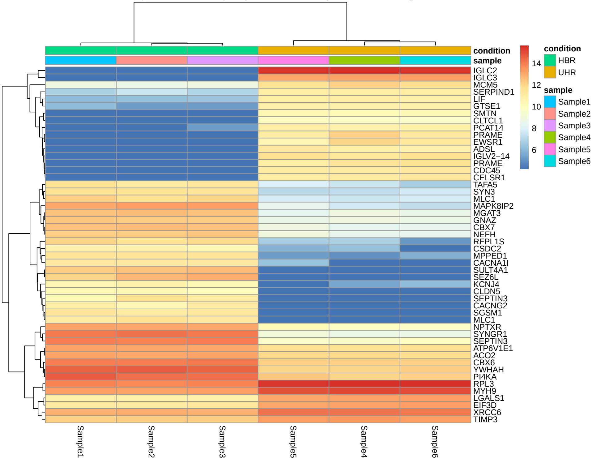
Heatmap of Differentially Expressed Genes (corrected labels)
