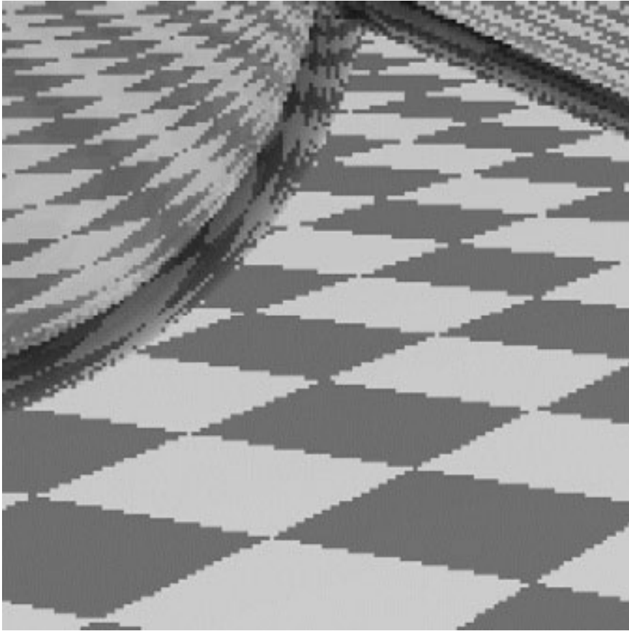
Jaggies
