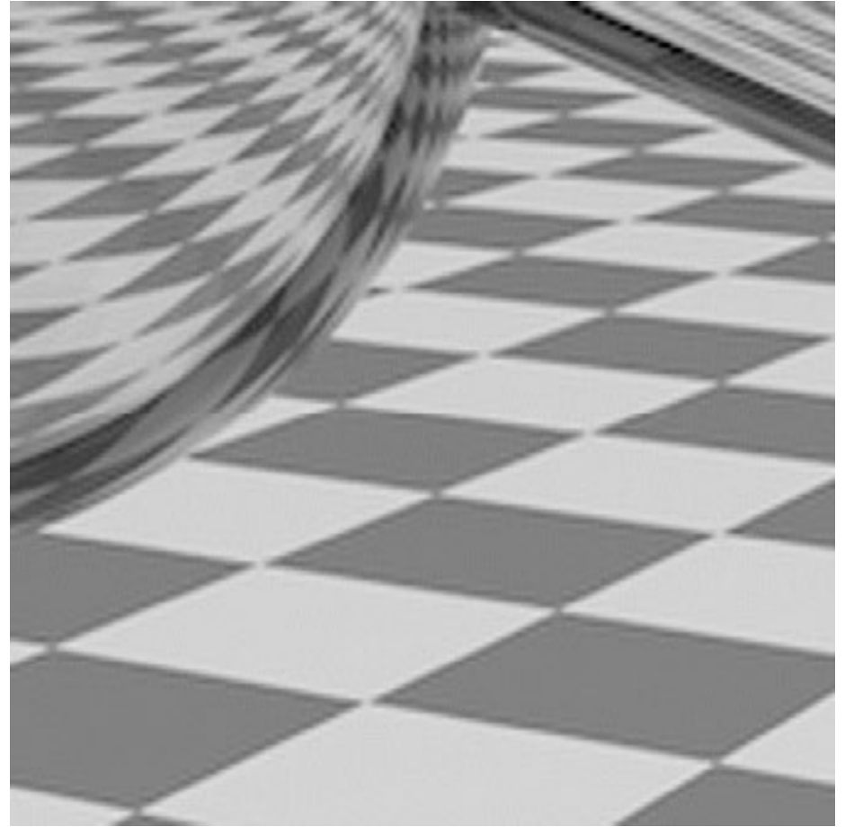
Pre-Filtered
