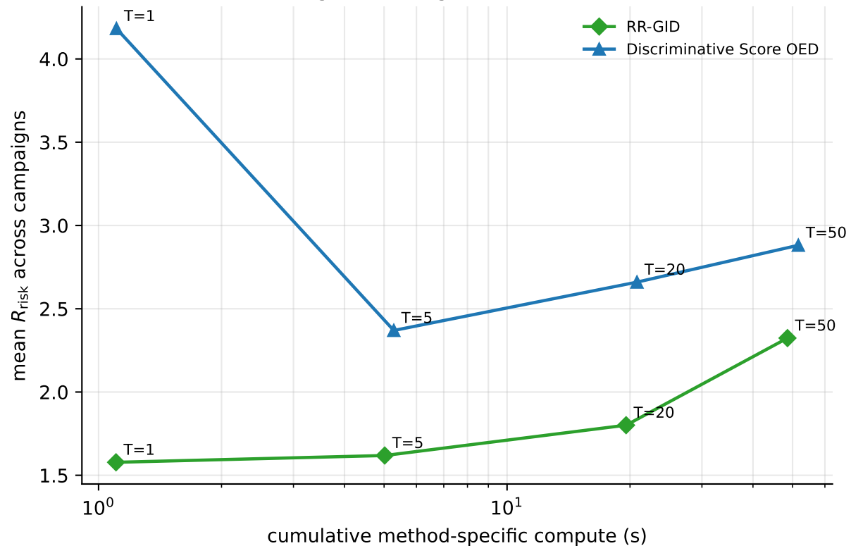
Figure 2(b): generator reuse
