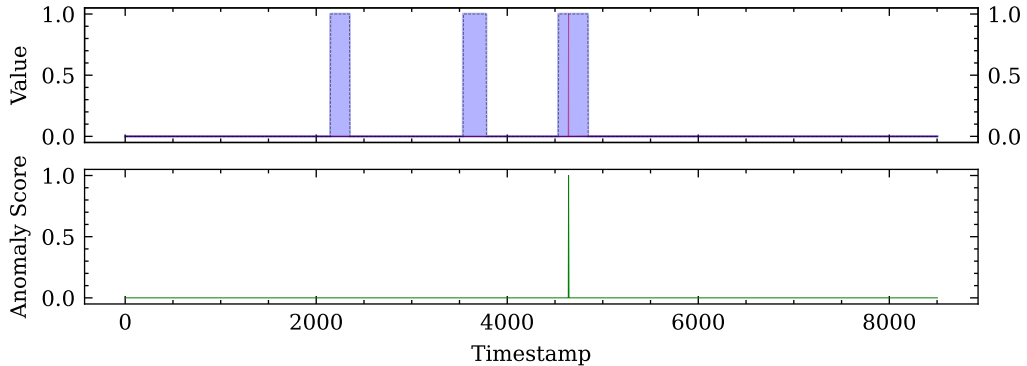
Dimension = 20
