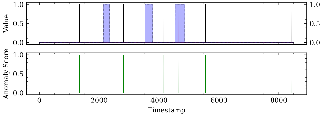
Dimension = 13
