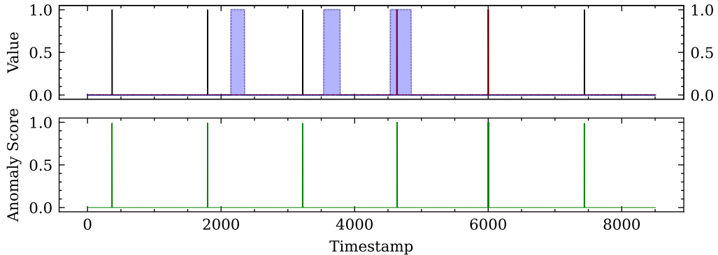
Dimension = 11
