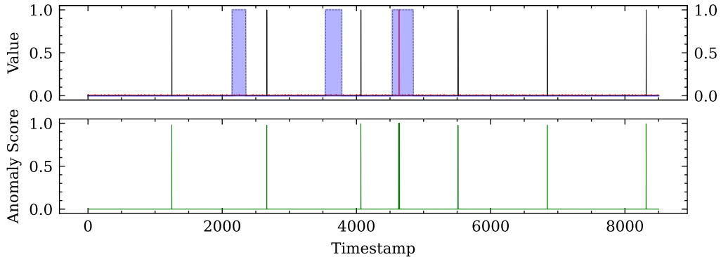
Dimension = 9
