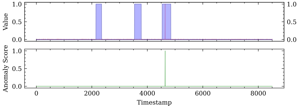
Dimension = 16
