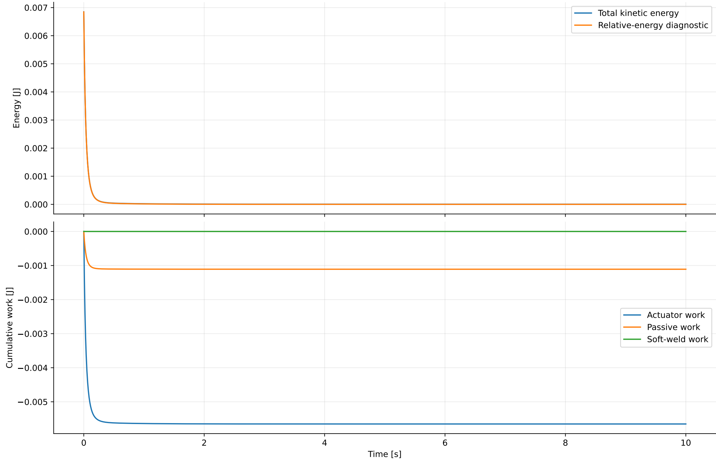
L_nominal — measured power accounting, including numerical residual
