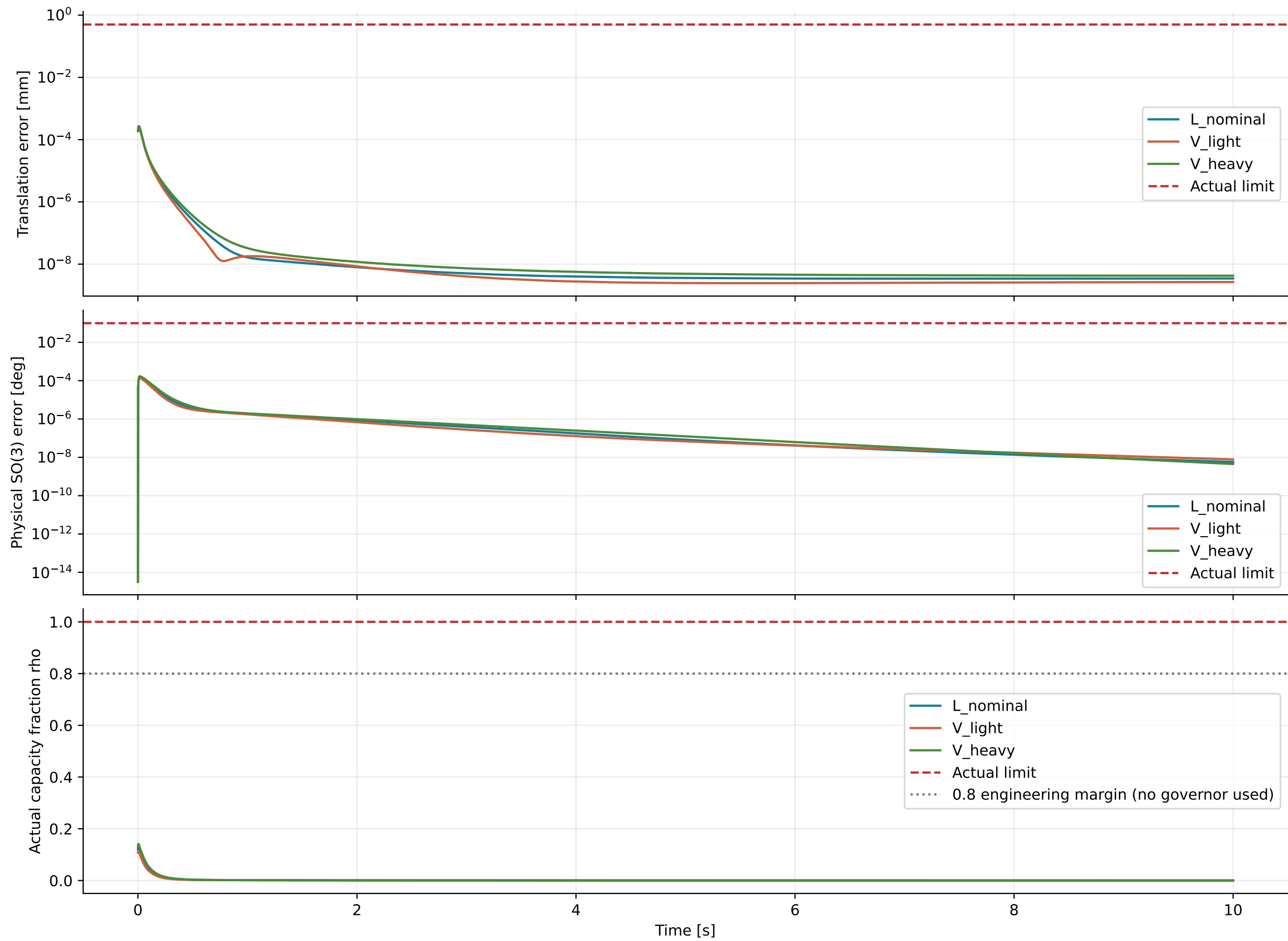
Interface holding and actual load — original hard limits
