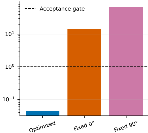
Terminal position error (mm)
