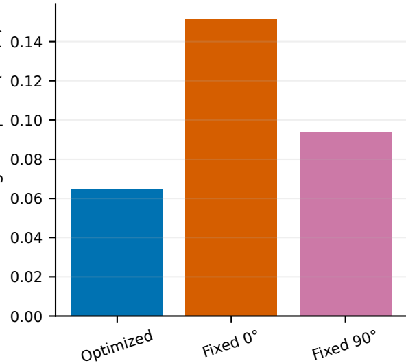
Peak base angular speed (rad/s)
