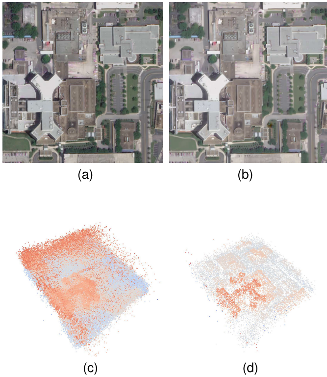
Fig. 6. Qualitative analysis of our GR module on scene JAX_068. (Top row) Final rendered images from (a) the base model and (b) our refined model. (Bottom row) Visualizes the corresponding Gaussian primitives (c) before and (d) after GR. Despite a significant reduction in primitives, the render quality is visually indistinguishable.
