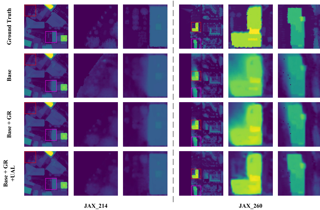
Fig. 5. Qualitative results of our ablation study on two representative scenes, JAX_214 and JAX_260. Each row visualizes the progressive improvement from our baseline (Base) to our full model (Base + GR + UAL). Within each result block, (left) full DSM, followed by two zoomed-in regions of interest. These two scenes were selected to demonstrate the complementary roles of our proposed components in addressing different types of geometric challenges. In JAX_214, the GR module (+GR) first cleans major artifacts from the complex building surfaces, after which the UAL module (+UAL) removes residual surface noise. Similarly, in JAX_260, our method first eliminates significant floating artifacts from the scene and then reduces fine-grained noise in the background.
