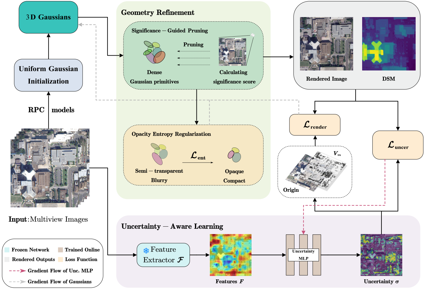
Fig. 1. Overview of our method. Our method takes multiview satellite images as input to reconstruct a high-fidelity 3-D scene represented by 3-D Gaussians. Input multiview images are processed using RPC models to define the scene bounds. Subsequently, a uniform volumetric initialization of 3-D Gaussians is applied to ensure the complete coverage [18]. To address geometric artifacts and view-inconsistent data common in satellite imagery, we introduce a two-pronged strategy. The GR module operates on the 3-D Gaussians directly, employing a significance-guided pruning step to remove redundant primitives, followed by an opacity entropy regularization \mathcal{L}_{ent} to resolve surface ambiguities and create a refined, geometrically consistent representation. In parallel, the UAL module leverages a pretrained feature extractor and a lightweight, online-trained MLP to predict a per-pixel uncertainty map. This map identifies unreliable regions, which are then down-weighted via the visibility map V_m in the rendering loss \mathcal{L}_{render} . Notably, the training of the uncertainty MLP and the 3-D Gaussians is decoupled; as indicated by different gradient flows, the uncertainty loss \mathcal{L}_{uncer} only updates the MLP, ensuring training stability.
