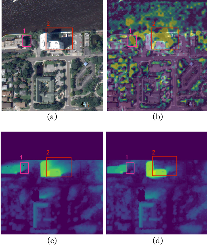
Fig. 2. Qualitative visualization of uncertainty on scene JAX_260. (a) Reference view. (b) Learned uncertainty mask ( 1 - V_m ). (c) DSM generated by the baseline model. (d) DSM generated by the baseline with UAL (Base + UAL). In our method, V_m acts as the confidence weight derived from the predicted uncertainty \sigma . We visualize 1 - V_m instead of raw \sigma to clearly illustrate the effective weight reduction applied during optimization. Consequently, yellow regions indicate high uncertainty, effectively capturing photometric inconsistencies in shadows (boxes 1 and 2), vegetation, and highly reflective water surfaces. In the bottom row, we specifically highlight the shadow regions (boxes 1 and 2) to demonstrate how down-weighting these areas eliminates artifacts and restores clean surface geometry.
