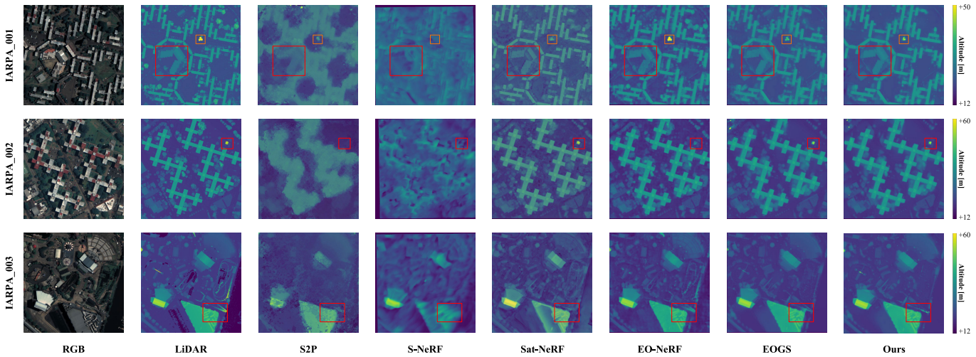
Fig. 4. Qualitative results of DSMs generated from IARPA. Each row displays the results for a single scene from all competing methods, while each column tracks the performance of one method across the different test scenes. Areas with significant differences are highlighted with bounding boxes. An altitude legend is provided on the right for reference. For visual context, the leftmost column provides a corresponding RGB image of each scene from a near-nadir perspective.
