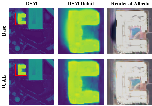
Fig. 8. Qualitative analysis of our UAL module on scene JAX_264. This figure compares the results from (top row) the baseline model against (bottom row) the baseline augmented with our UAL module to isolate its contribution. The module’s effectiveness is twofold. First, it enhances geometric accuracy, as seen in the DSM detail column, where the building edges in the bottom row are significantly sharper than in the top row. Second, it corrects major rendering artifacts. In the rendered albedo column, the large, dark artifact present on the building facade in the baseline result is successfully removed after applying the uncertainty module.
