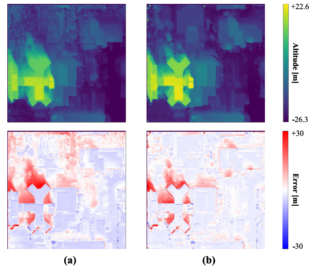
Fig. 7. Qualitative analysis of the GR module under a five-view training setting. (Top row) Compares the generated DSMs from (a) baseline model and (b) our model with GR module. (Bottom row) Visualizes their respective error maps against the ground truth. Our method significantly suppresses the floating artifacts and refines the geometric details. Both DSMs and error maps are rendered with shared colorbars for fair comparison.
