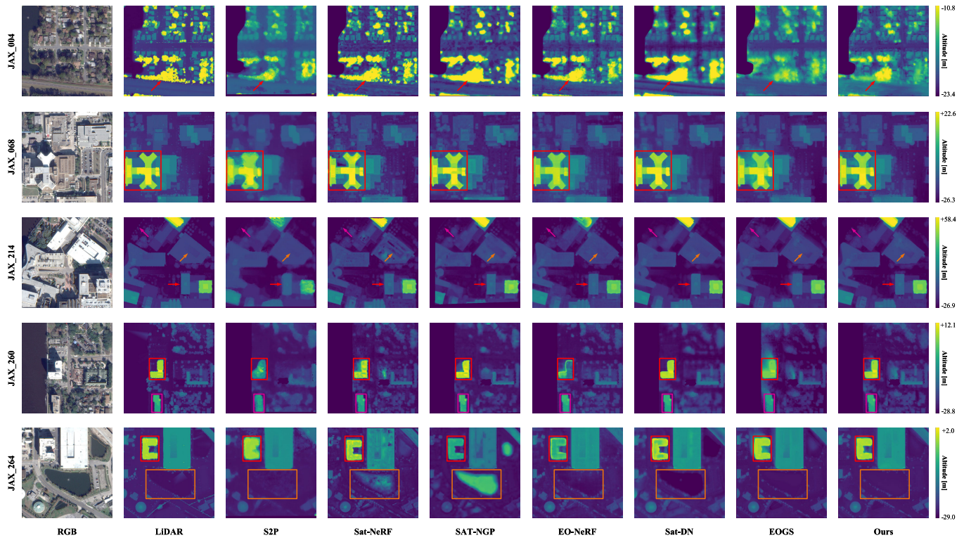
Fig. 3. Qualitative results of DSMs generated from JAX. Each row displays the results for a single scene from all competing methods, while each column tracks the performance of one method across the different test scenes. Areas with significant differences are highlighted with bounding boxes, while arrows are used to indicate specific discrepancies in irregular regions unsuitable for boxes. An altitude legend is provided on the right for reference. For visual context, the leftmost column provides a corresponding RGB image of each scene from a near-nadir perspective.
