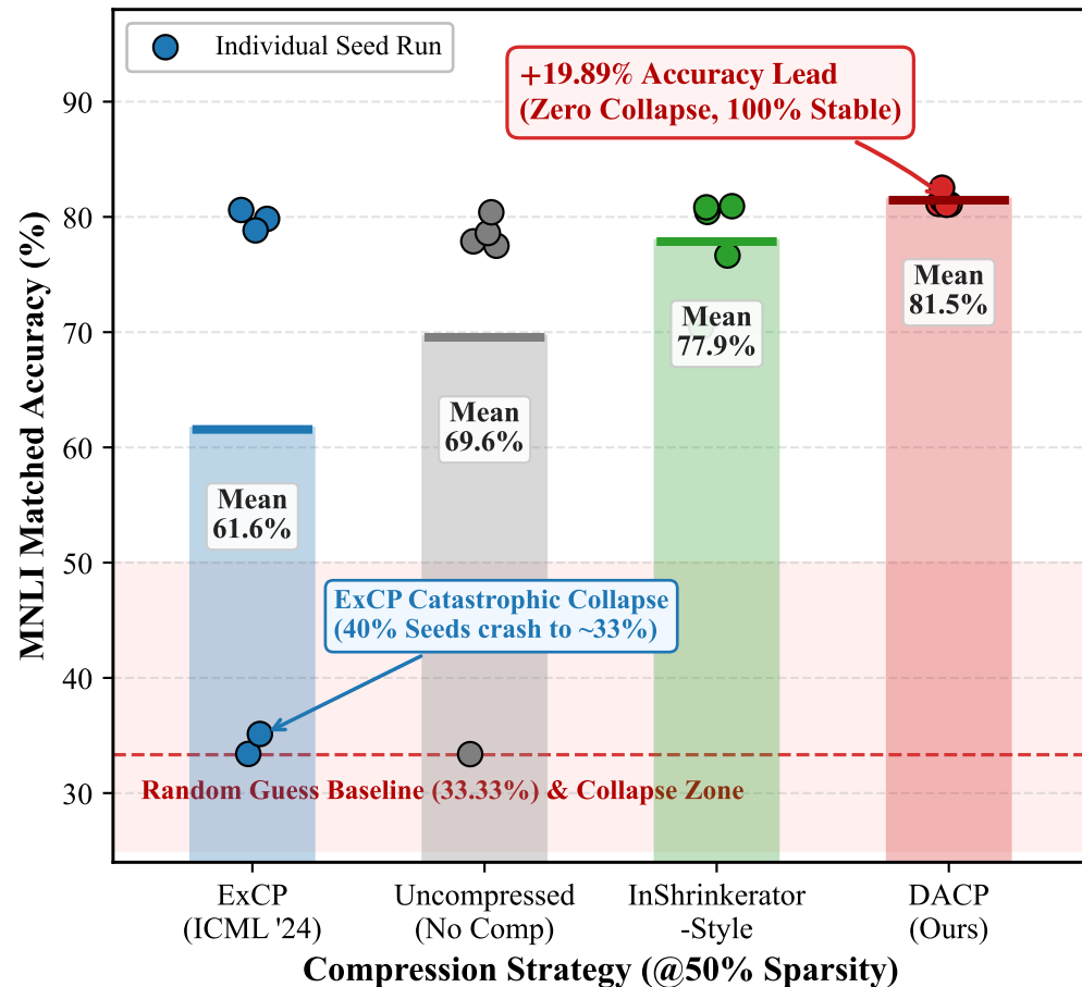
(b) Downstream Robustness: Zero-Collapse Defense (BERT-Large MNLI)
