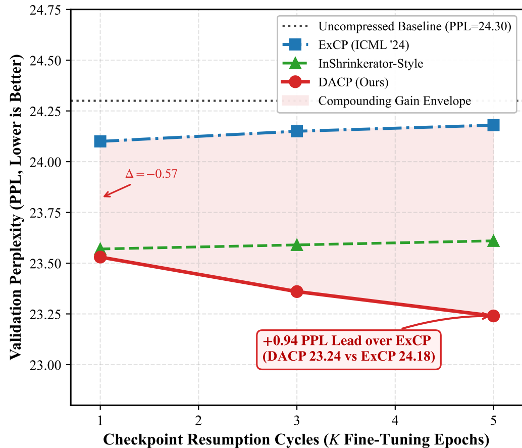
(a) Continuous Resumption: Compounding Quality Advantage
