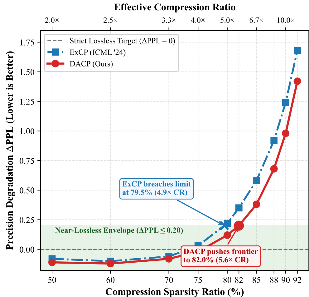
(a) Fine-Grained Precision Degradation ( \Delta\text{PPL} )
