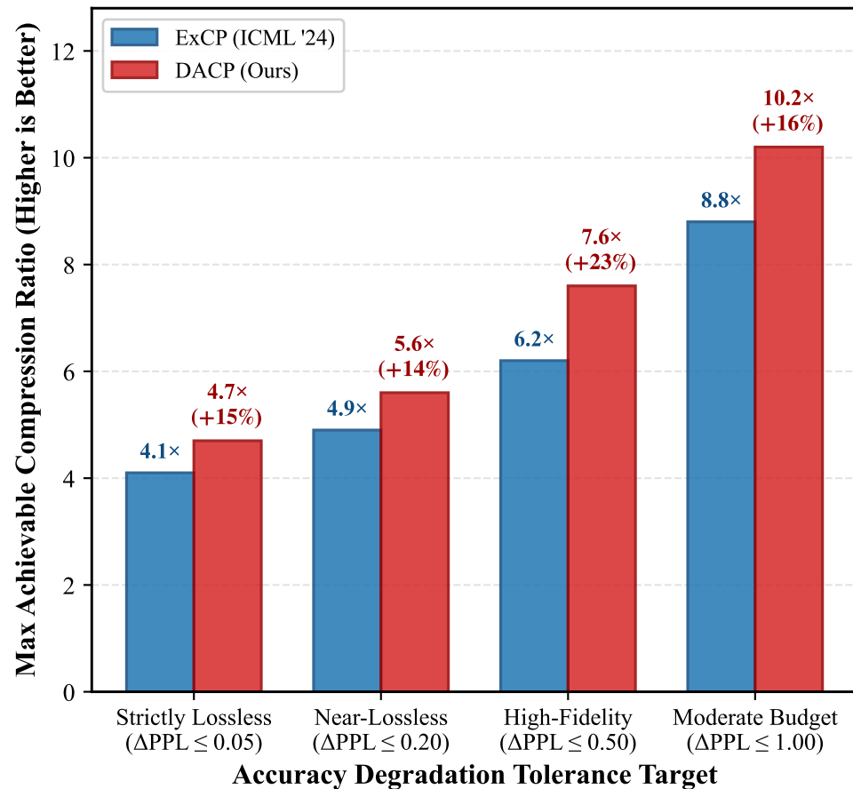
(b) Max Compression Ratio under Quality Tolerance
