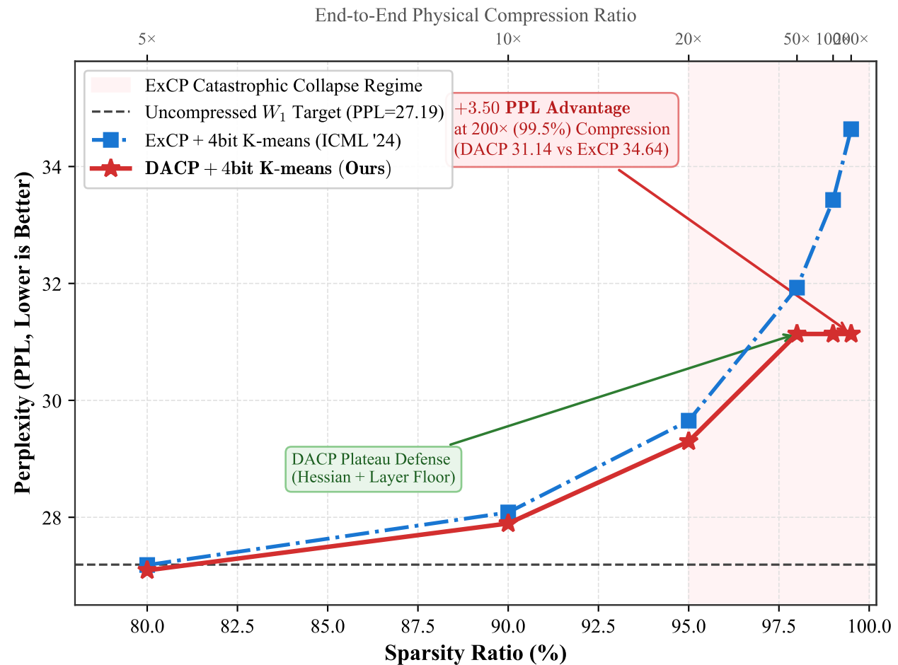
(b) End-to-End Compression (Pruning + 4-bit Quantization)
