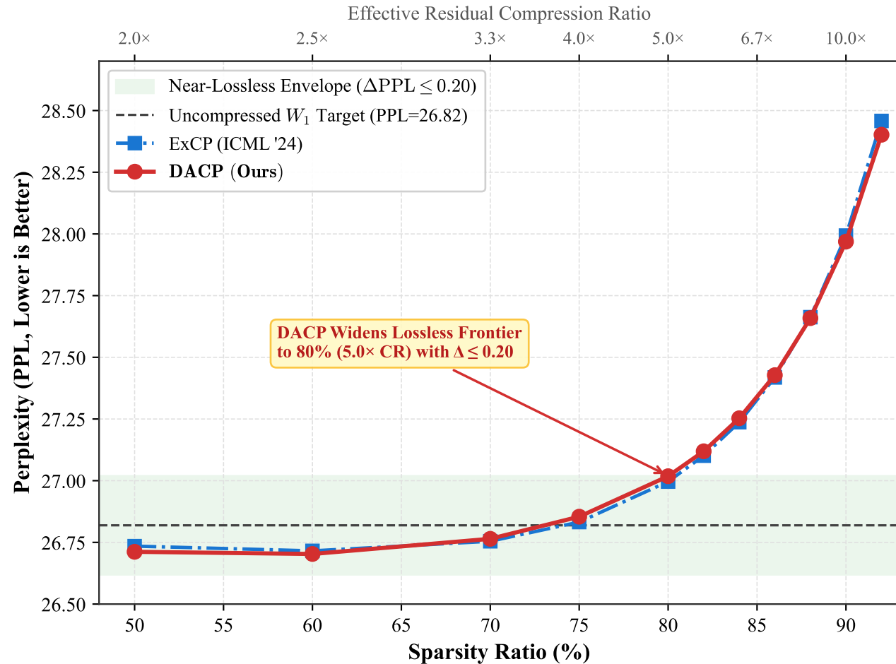
(a) Fine-Grained Near-Lossless Compression Frontier
